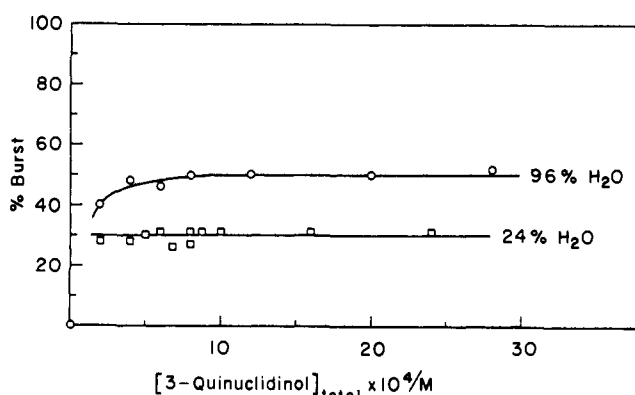
Figure 4. Effect of solvent on the percent of 3,4-dinitrophenoxide ion release that appears as a burst when 3,4-dinitrophenyl chloroformate is reacted with 3-quinuclidinol in the presence of 10^{-3} M p -acetophenol (total) in 4% tetrahydrofuran (O) and in 4% tetrahydrofuran plus 72% acetonitrile (by volume) (□). The solutions were buffered with 0.01 M borate, 20% base.
