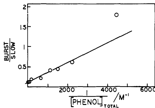
Figure 7. The ratio of burst to slow release of 4-nitrophenoxide ion as a function of the reciprocal of the phenol concentration, in the partitioning of the intermediate formed from 1-(4-nitrophenyloxycarbonyl)-3-methylimidazolium ion at 25 °C in 0.0024 M borate buffer, pH 8.5.
